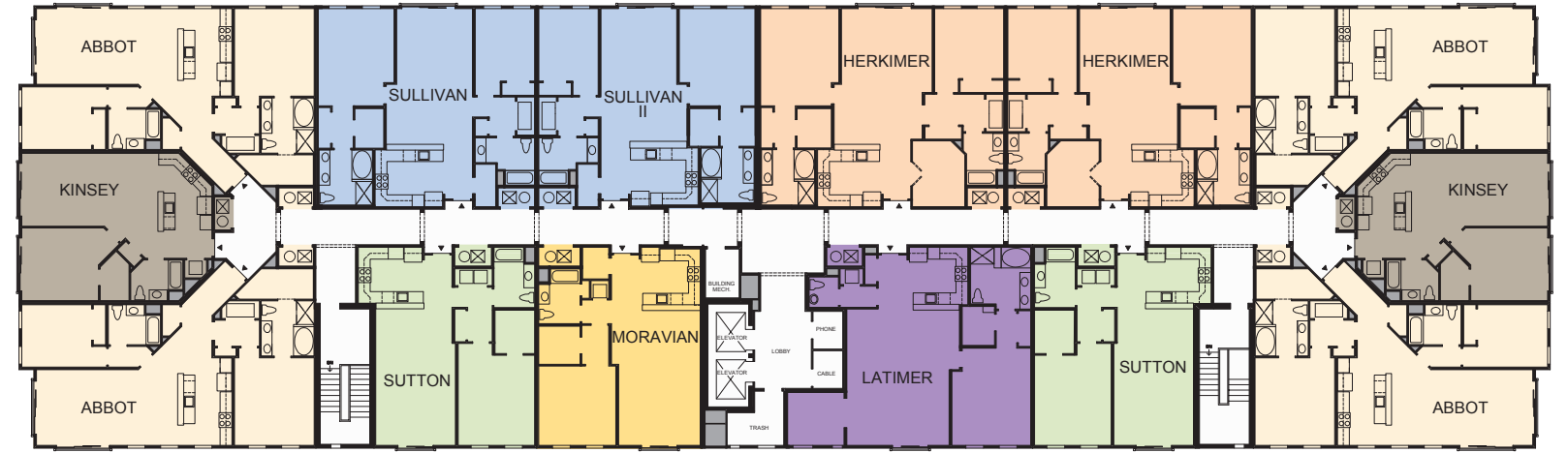
FOURTH FLOOR
