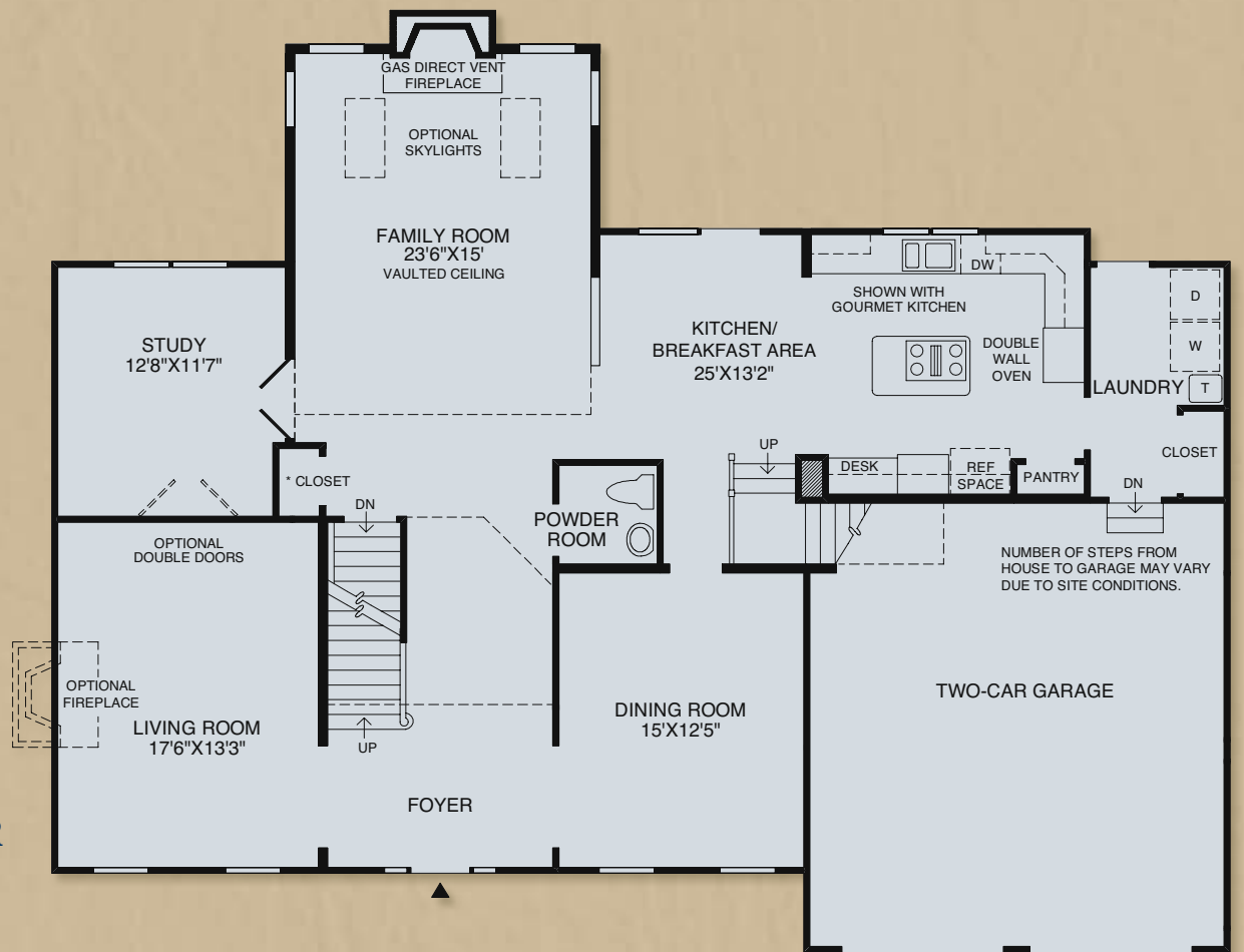
FIRST FLOOR
