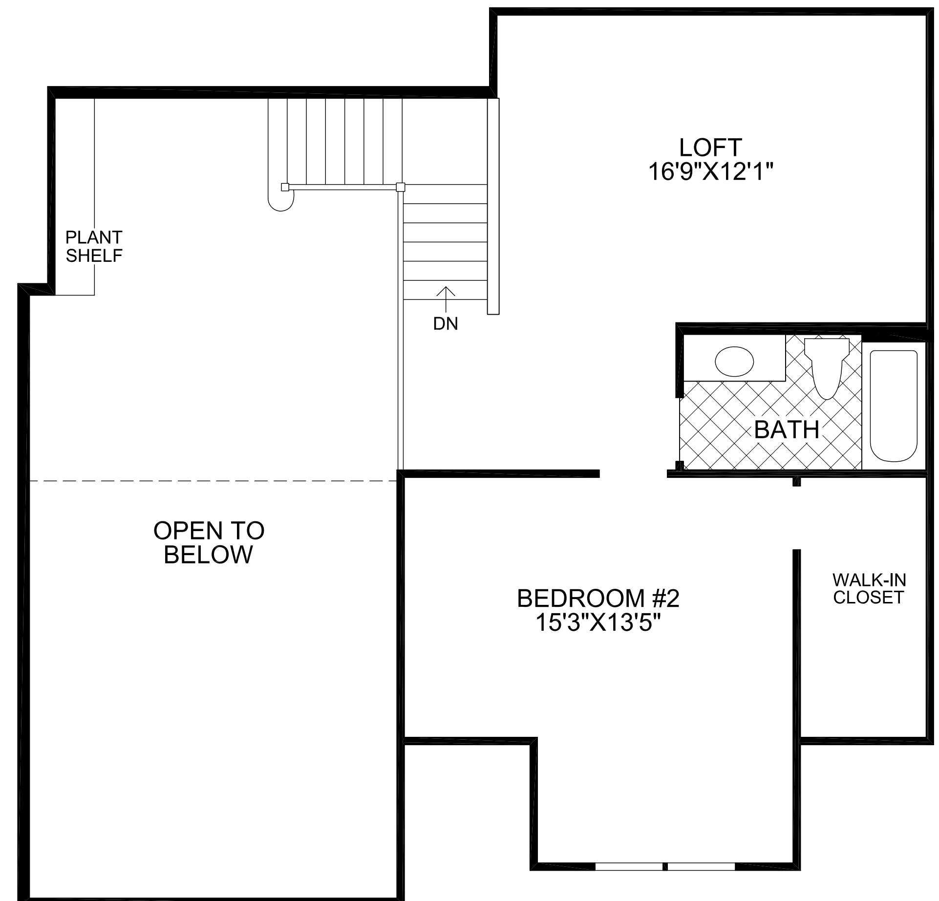
SECOND FLOOR
