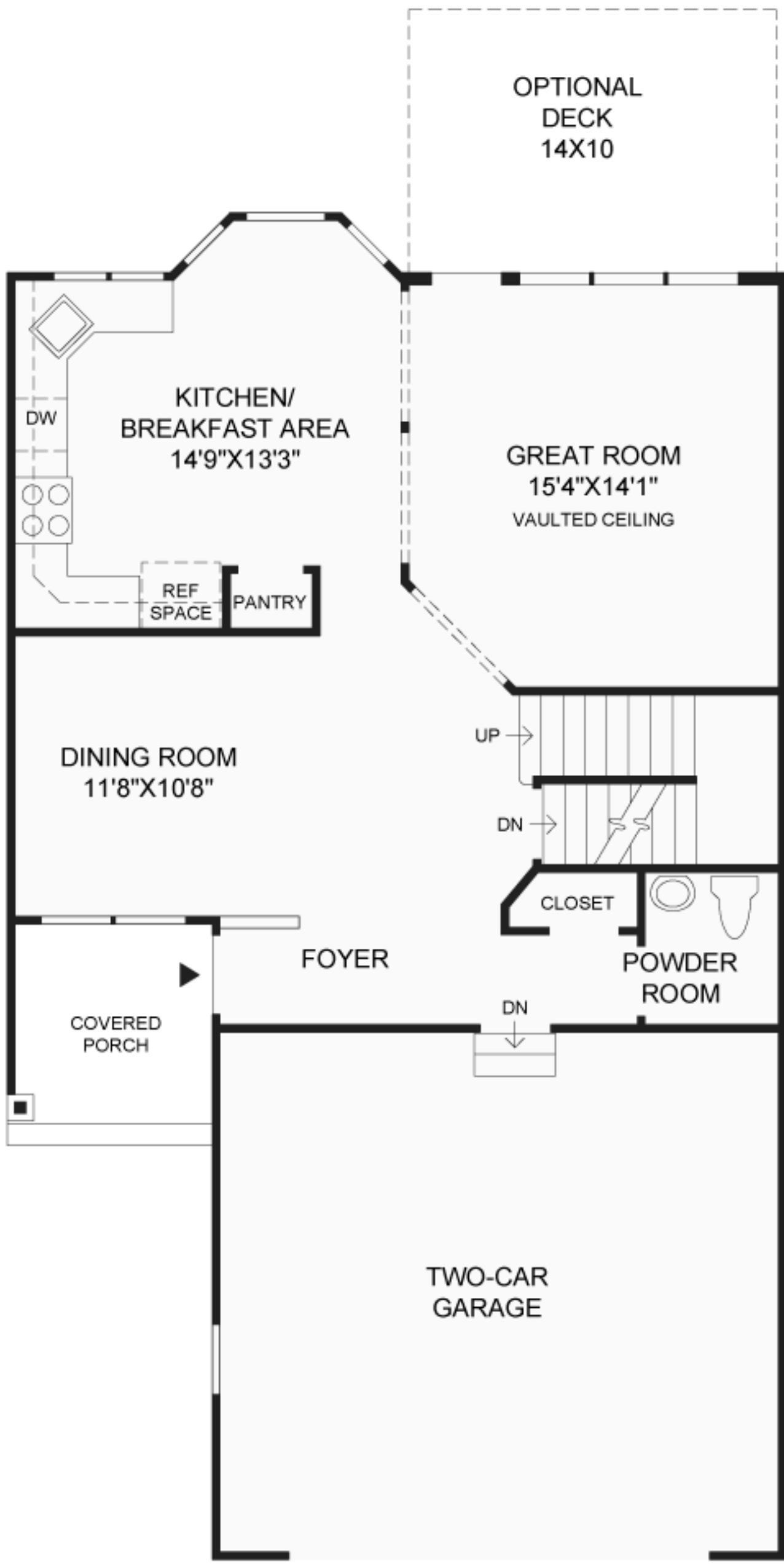
FIRST FLOOR
