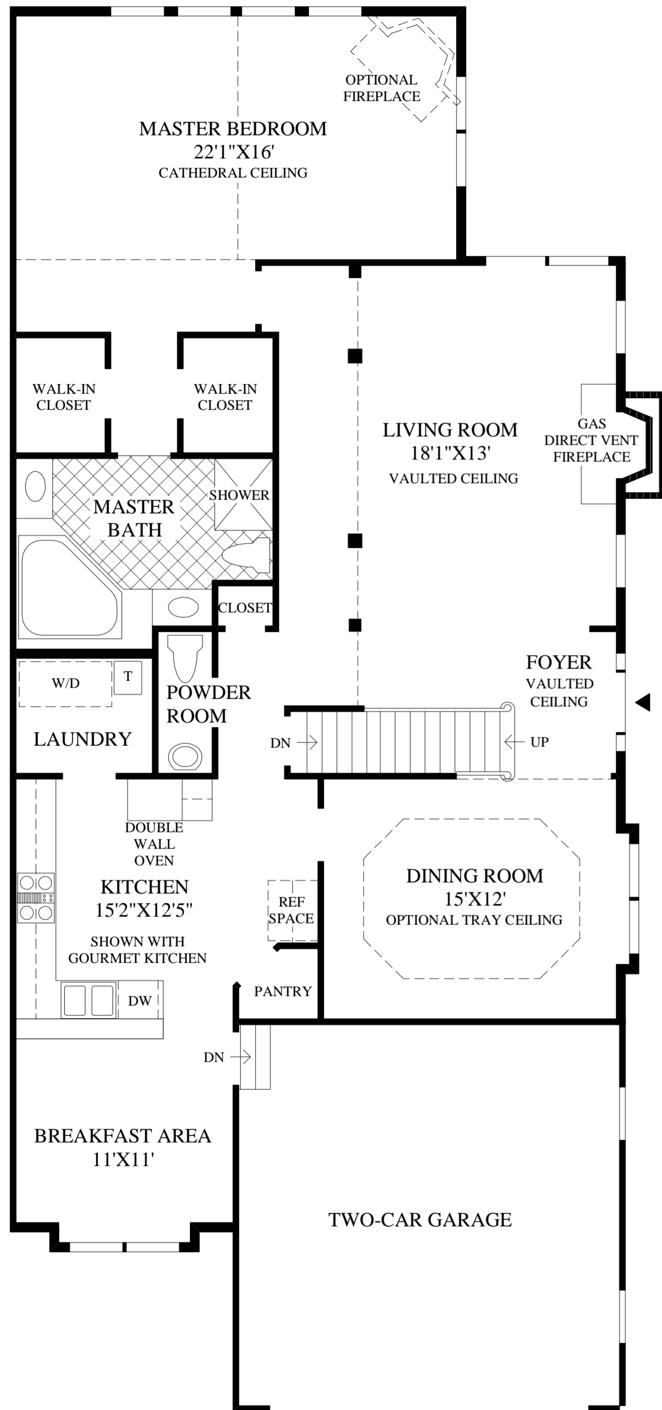
First Floor
