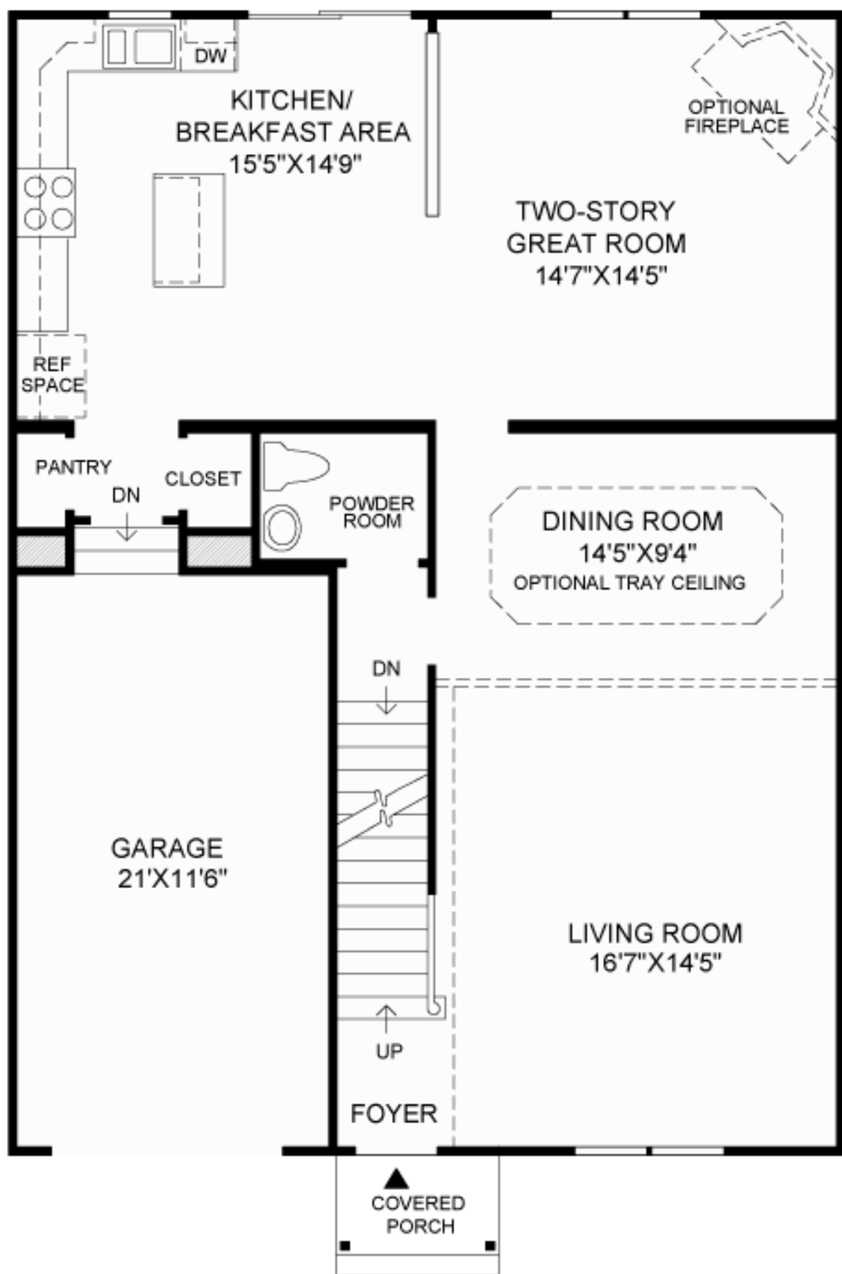
FIRST FLOOR
