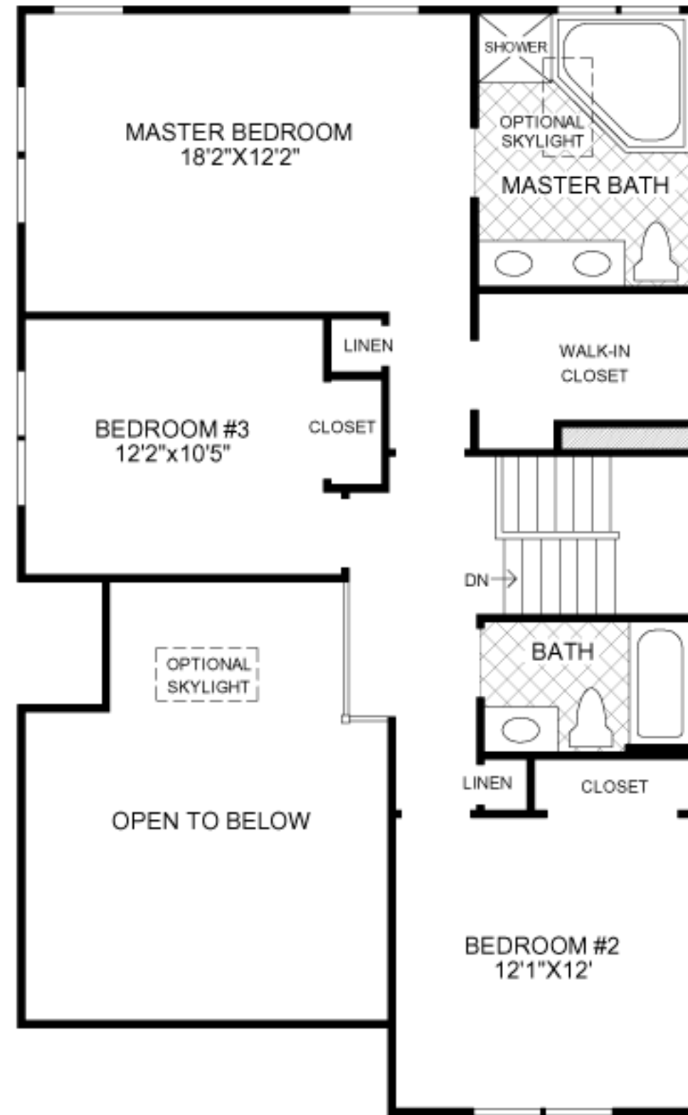
SECOND FLOOR
