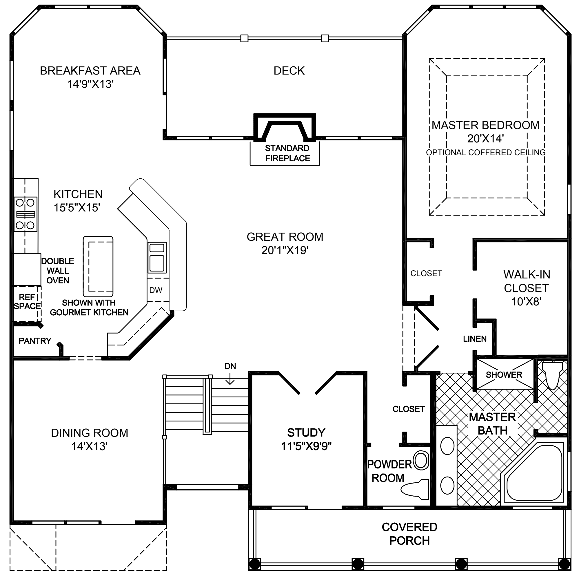
SECOND FLOOR
