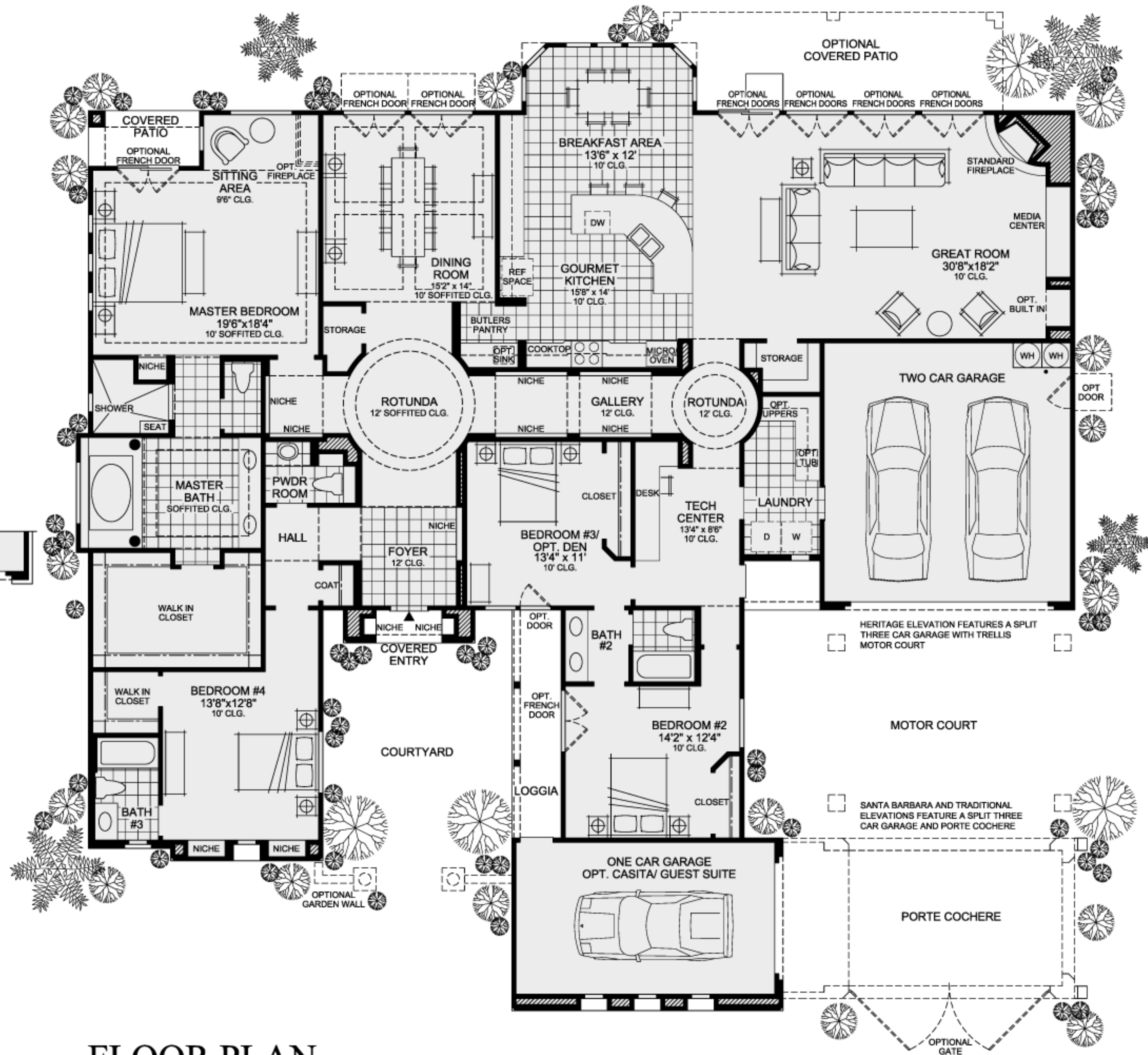
FLOOR PLAN
